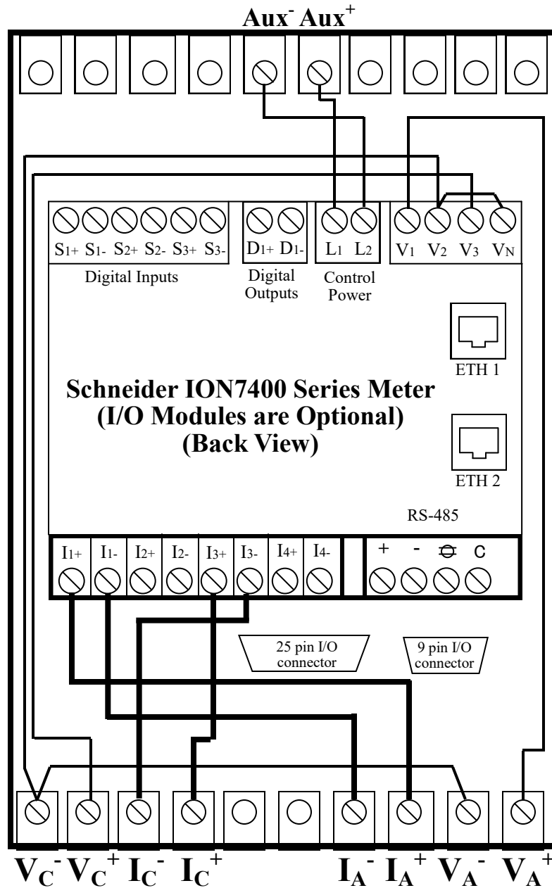
Back View
