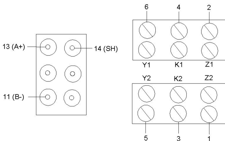
Back View of EPM 5100 Case
