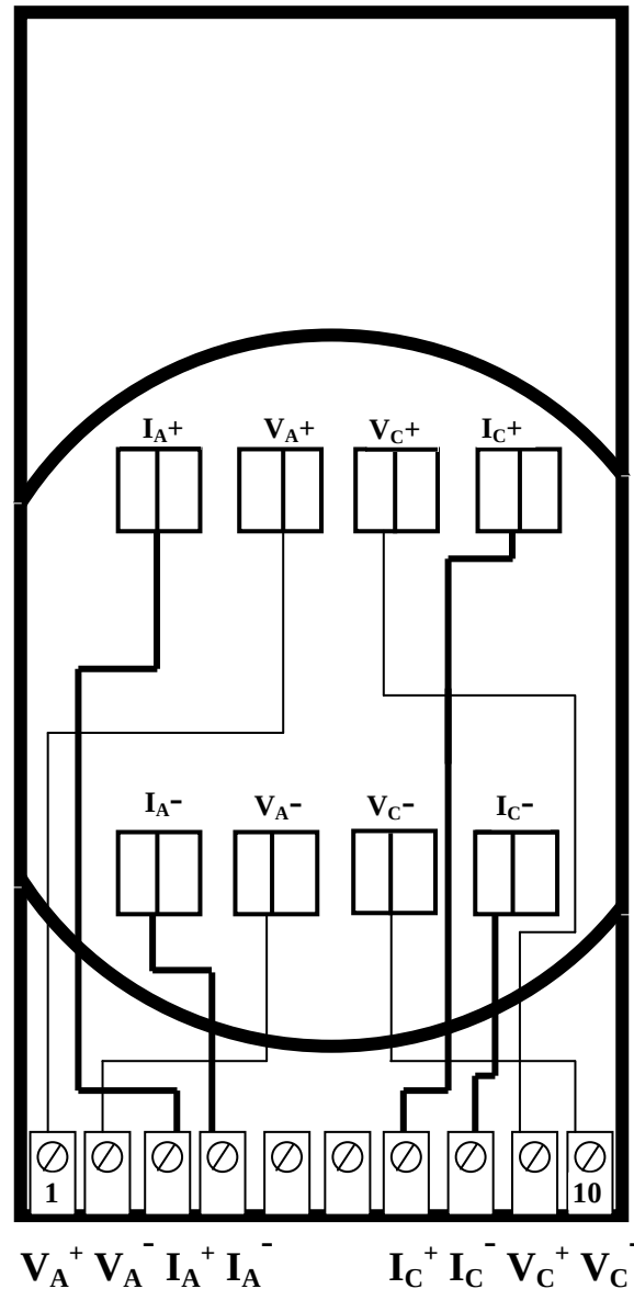
Front view of Panel Adapter
