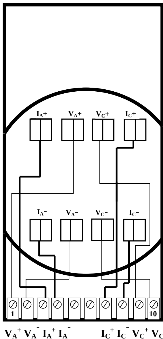
Front view of Retrofit Panel Adapter
