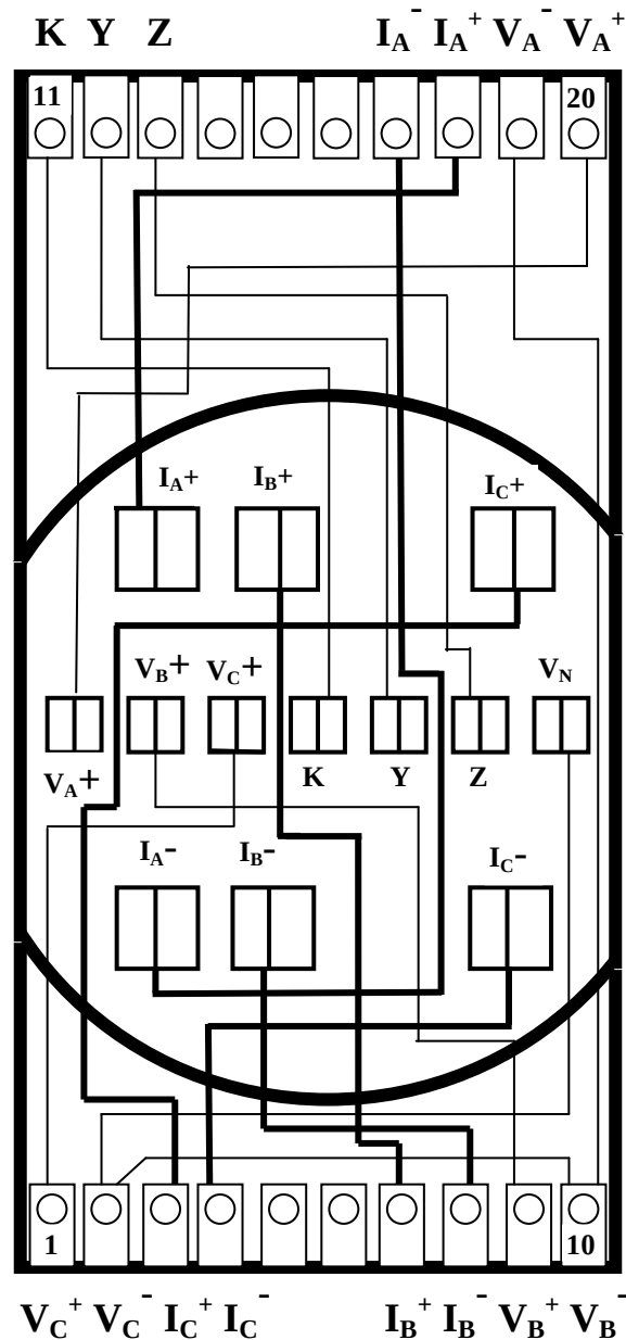
Front view of Retrofit Panel Adapter
