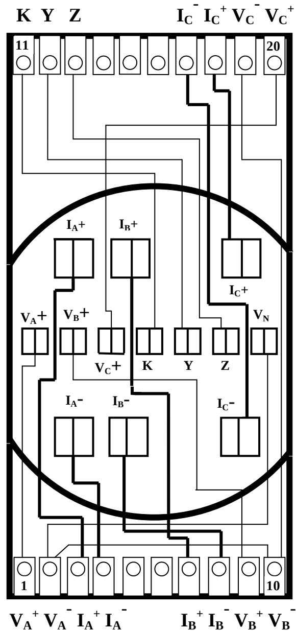
Front view of Retrofit Panel Adapter
