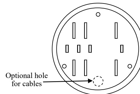
Base of the PS9 Socket Adapter
