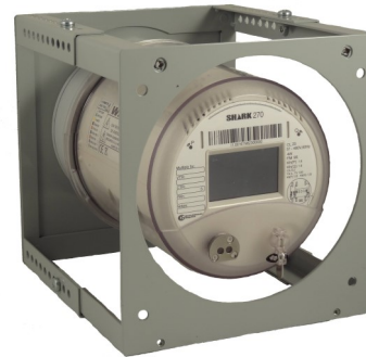
Flush Mount Adapter with Shark 270 meter Expanded
