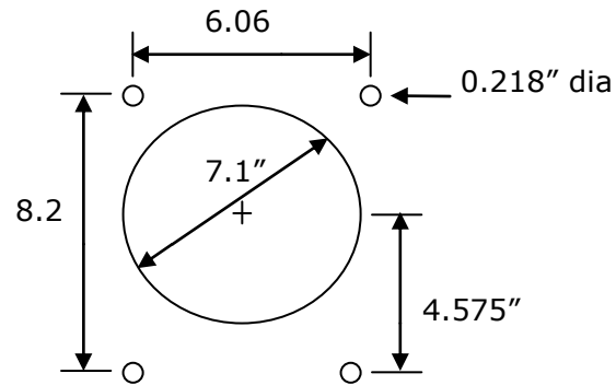
Panel Cutout
