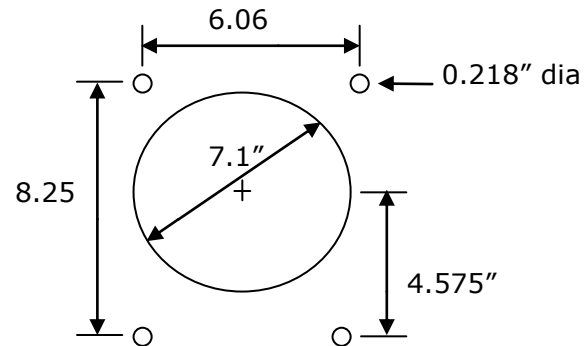
Panel Cutout
