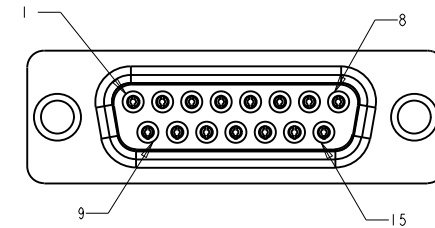
VIEW FROM BACK OF METER
