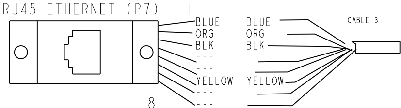
CONNECTORS PLUG
