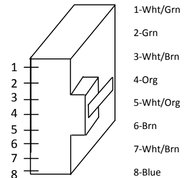
RJ45 Ethernet
