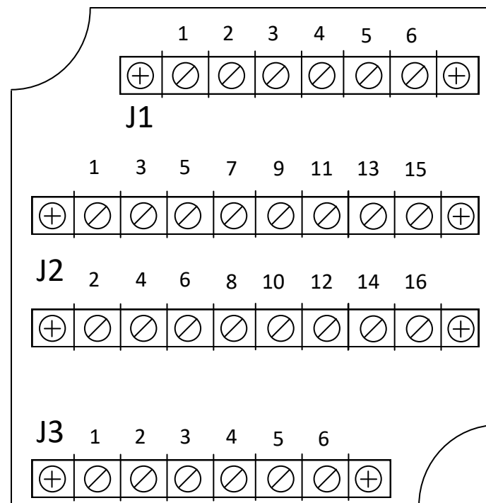
Back of GE ES Meter Case
