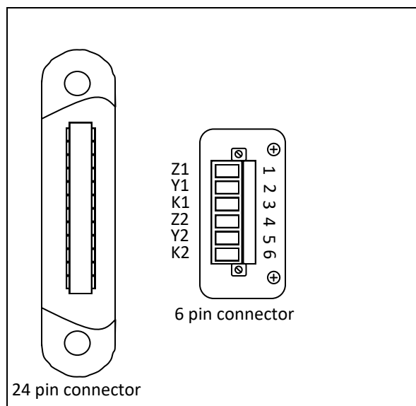
ESK Bracket
