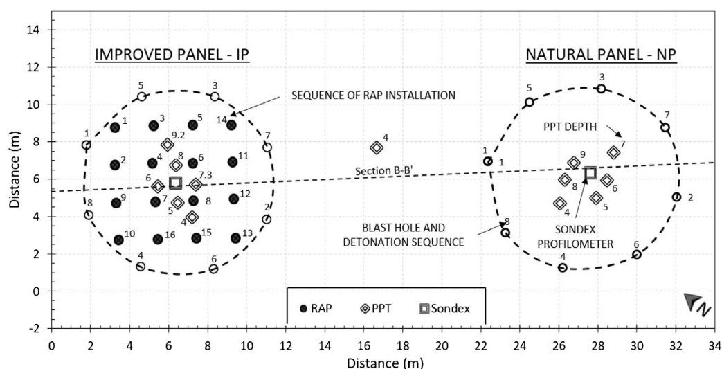
Fig. 3. Locations of blast holes, RAP columns, pore pressure transducers (PPTs), and profilometers for the natural and improved panels. Numbers by blast holes indicate detonation sequence, numbers by RAP columns indicate construction sequence, numbers by PPTs indicate depth.
