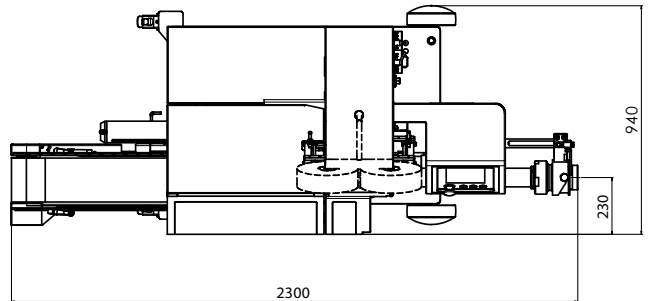
Top view (dimension in mm)
