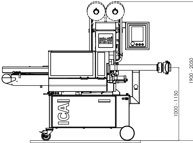
Front view (dimension in mm)
