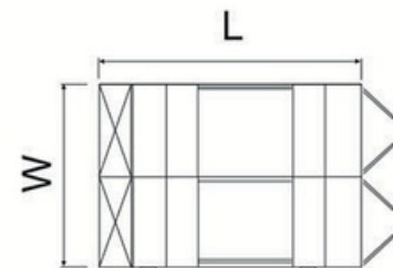
CPT-205 (2 Bay x CPT-105)
