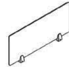
APBS-60 W60xD3.3xH36.5 cm. APBS-70 W70xD3.3xH36.5 cm. APBS-100 W110xD3.3xH36.5 cm.
