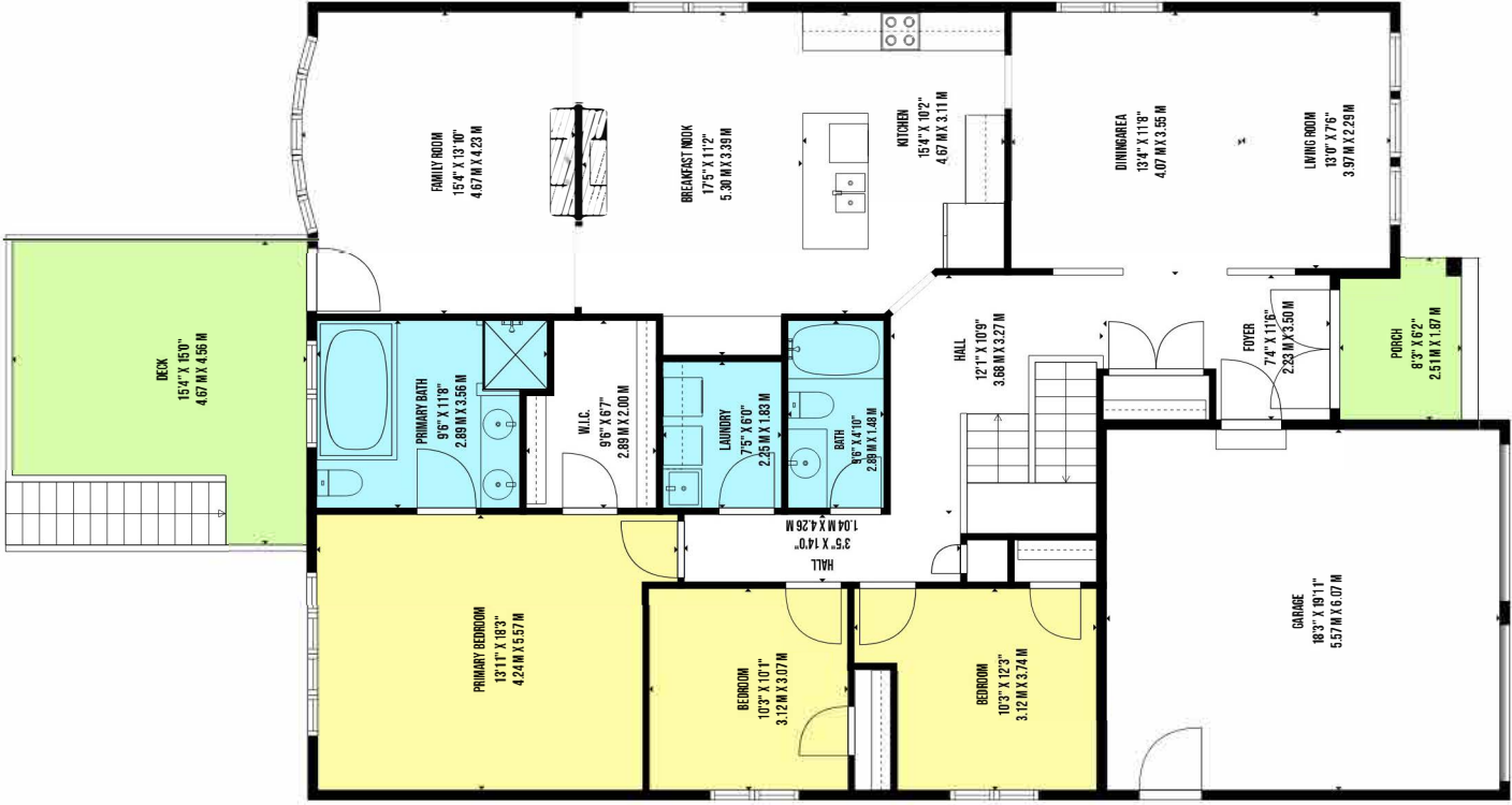
1ST FLOOR
