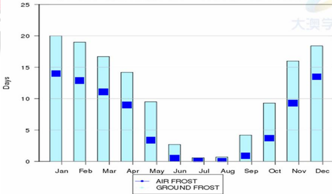
Average annual number of days of air and ground frost (1981-2010) at Lough Navar Forest (126 metres amsl)
