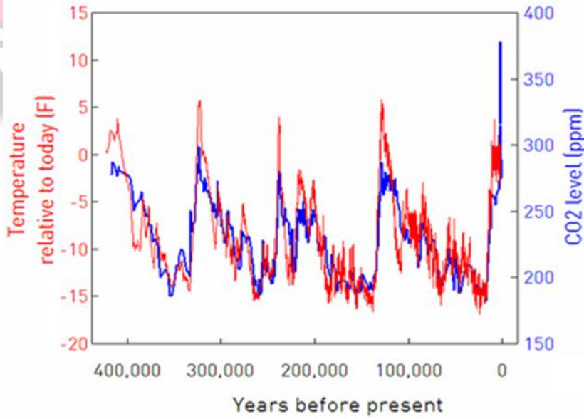
Temperature and CO2 for Last 400,000 Years
