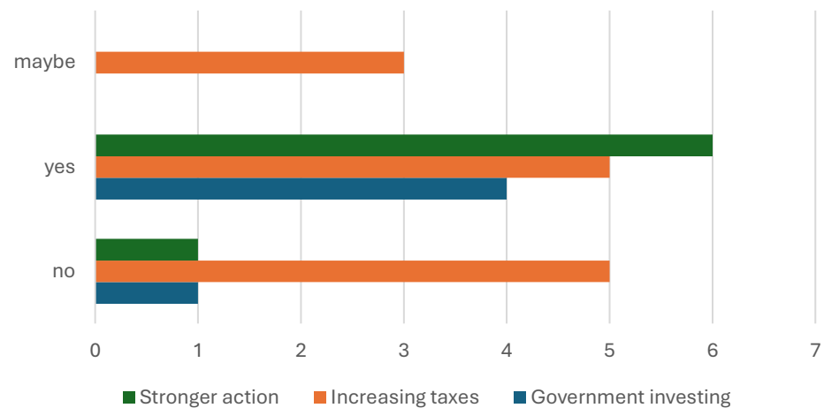
Graph #2: Climate Change
