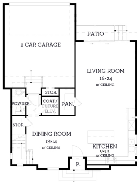
First Floor 935 sq.ft.
