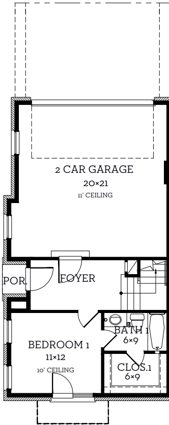
First Floor 392 sq.ft.
