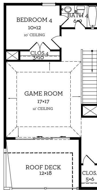
Fourth Floor 686 sq.ft.
