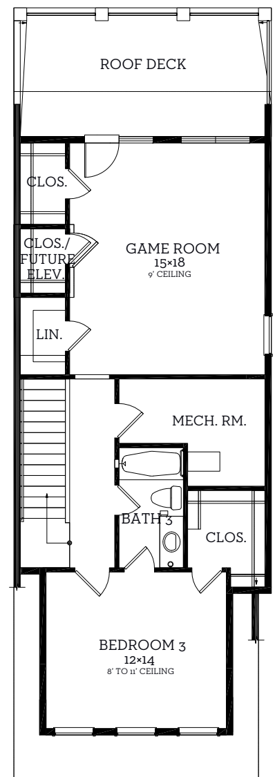
Third Floor 730 sq ft.
