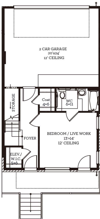
First Floor 492 sq.ft.
