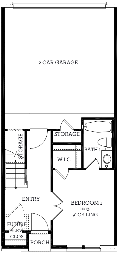
First Floor 420 sq.ft
