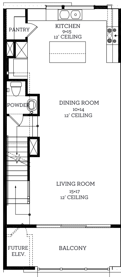
Second Floor 741 sq.ft
