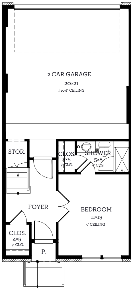
First Floor 389 sq.ft.
