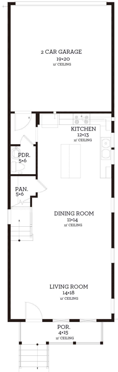
First Floor 713 sq.ft.
