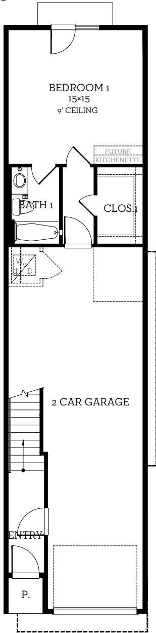
First Floor 450 sq.ft.
