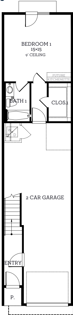
First Floor 450 sq.ft.
