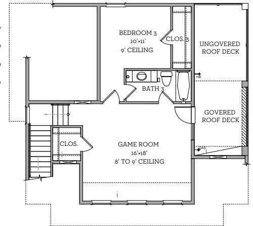
Third Floor 590 sq.ft.
