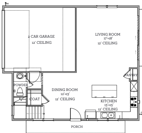
First Floor 829 sq.ft.
