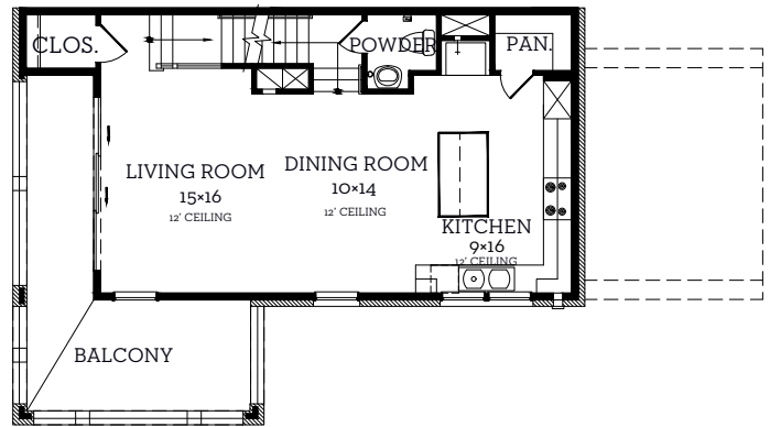
Second Floor 780sq.ft.
