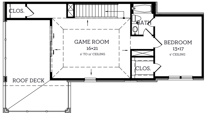
Fourth Floor 835 sq.ft.
