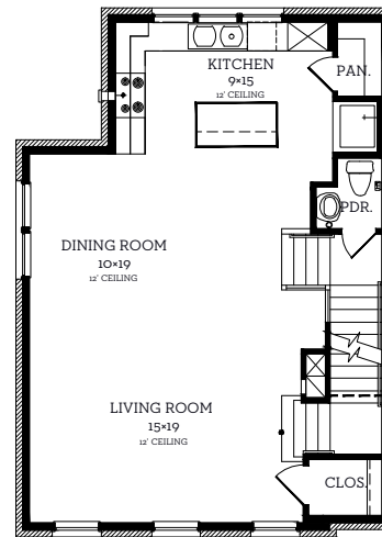
Second Floor 864 sq.ft.
