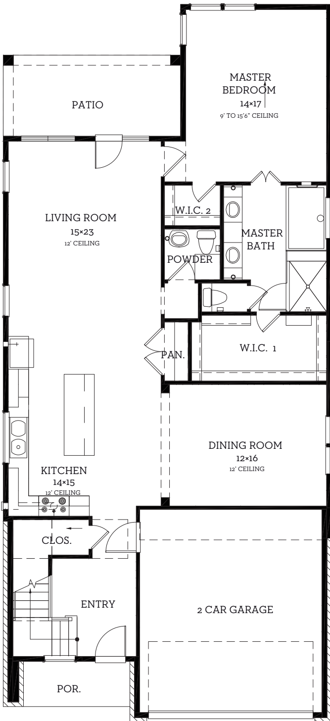
First Floor 1590 sq.ft.
