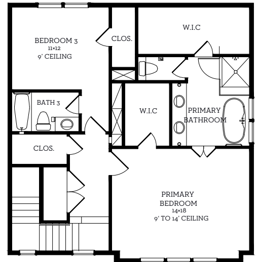
Third Floor 931 sq.ft
