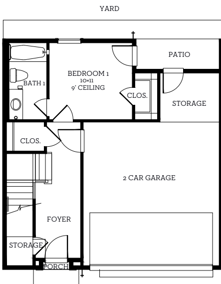
First Floor 419 sq.ft
