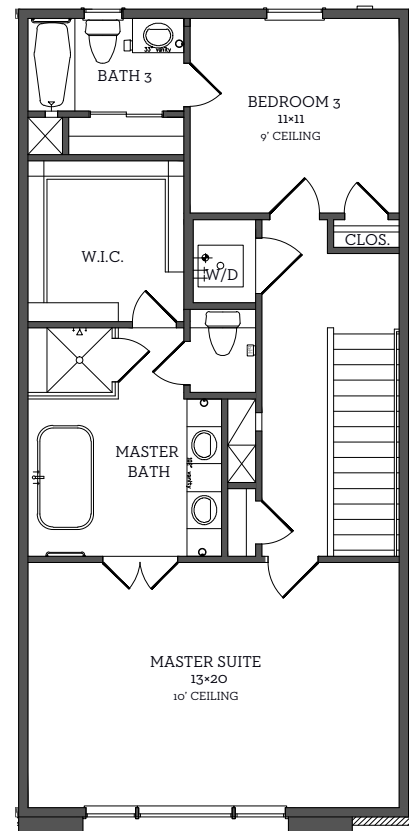
Third Floor 926 sq.ft.
