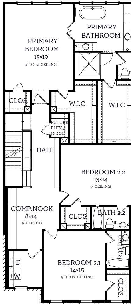
Second Floor 1905 sq.ft.
