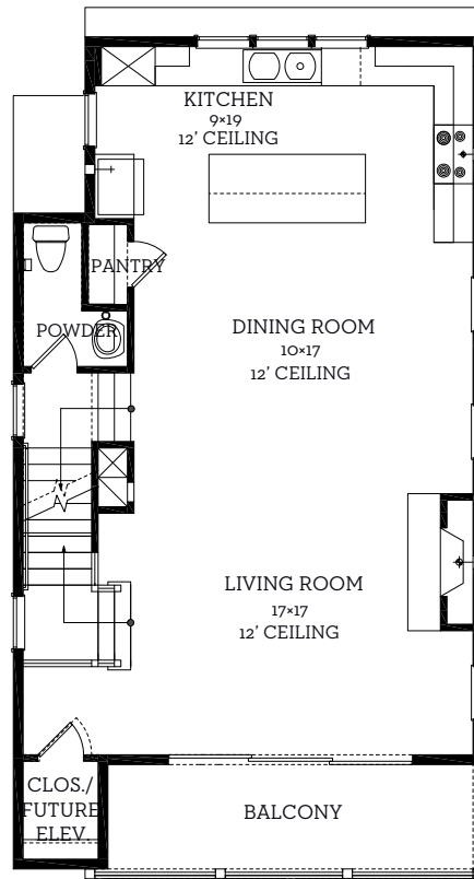
Second Floor 885 sq.ft
