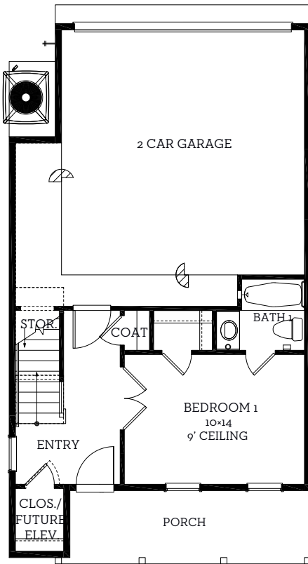
First Floor 392 sq.ft
