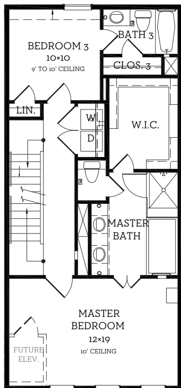
Third Floor 860 sq.ft.
