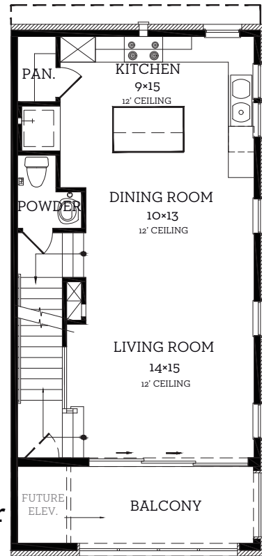
Second Floor 690 sq.ft.
