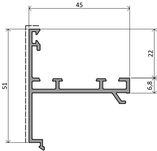
NX3706 | 0,586 Kg/m
