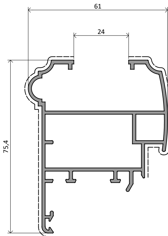
NX3548 | 1,246 Kg/m
