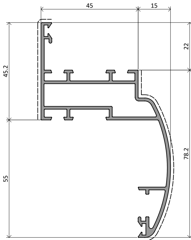
NX4270 | 1,163 Kg/m
