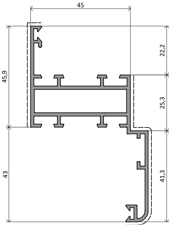
NX3554 | 1,115 Kg/m
