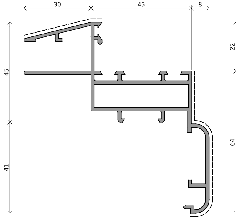
NX3707 | 1,328 Kg/m
