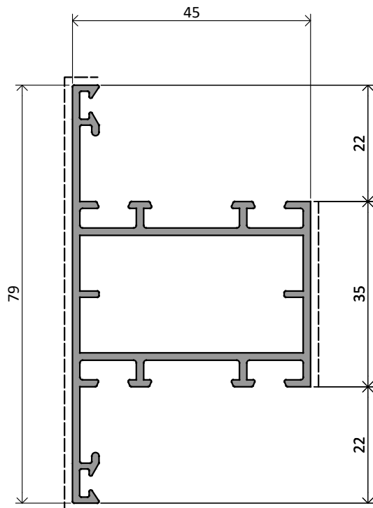
NX2766 | 1,031 Kg/m
