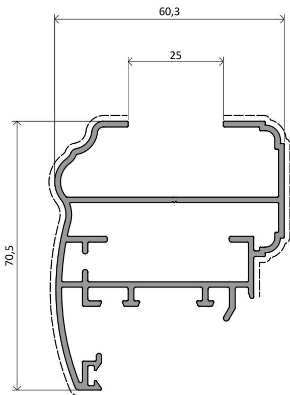
NX10604 | 1,293 Kg/m
