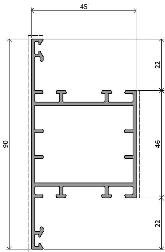
NX43 | 1,170 Kg/m
