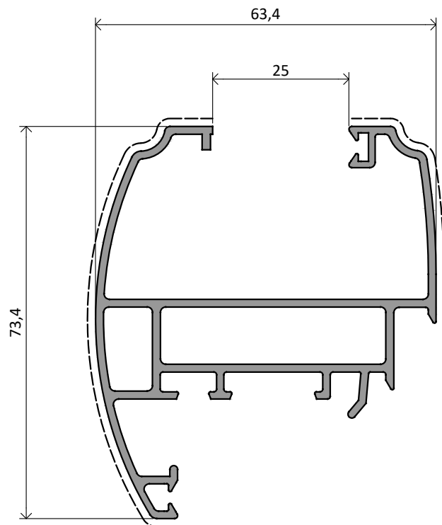
NX3795 | 1,255 Kg/m
