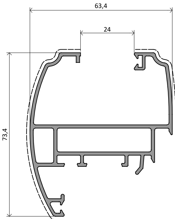
NX3766 | 1,291 Kg/m
