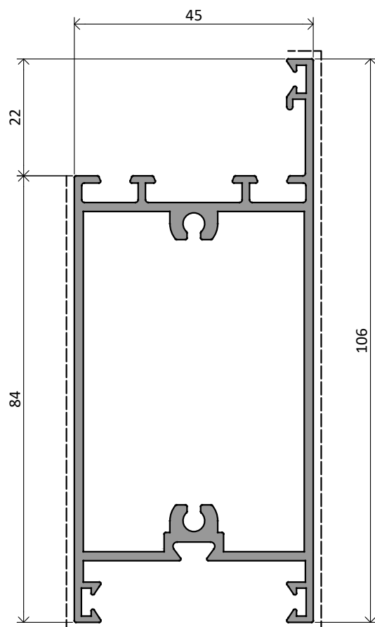
NX809 | 1,623 Kg/m
