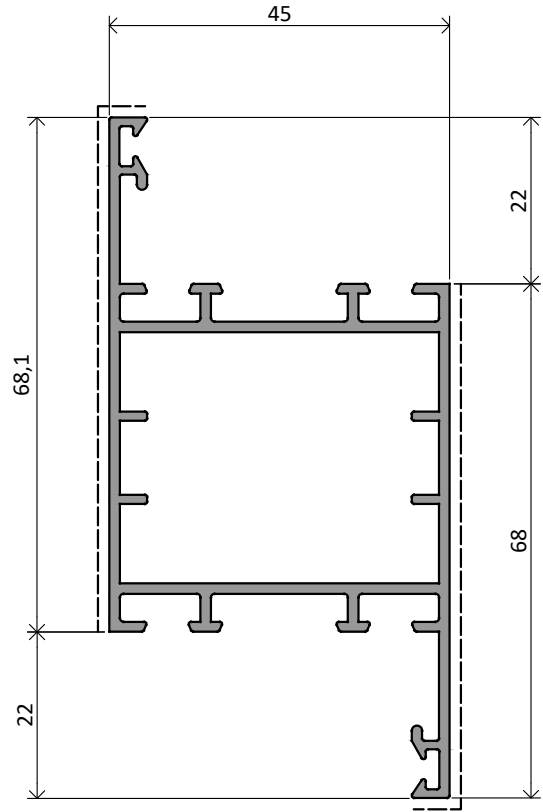
NX42 | 1,215 Kg/m
