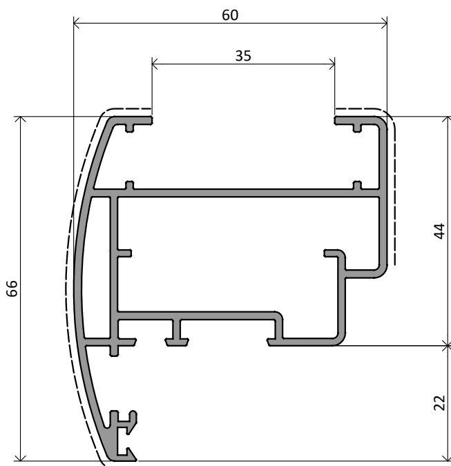
NX4272 | 1,242 Kg/m
