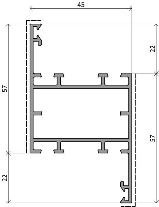
NX3705 | 1,023 Kg/m
