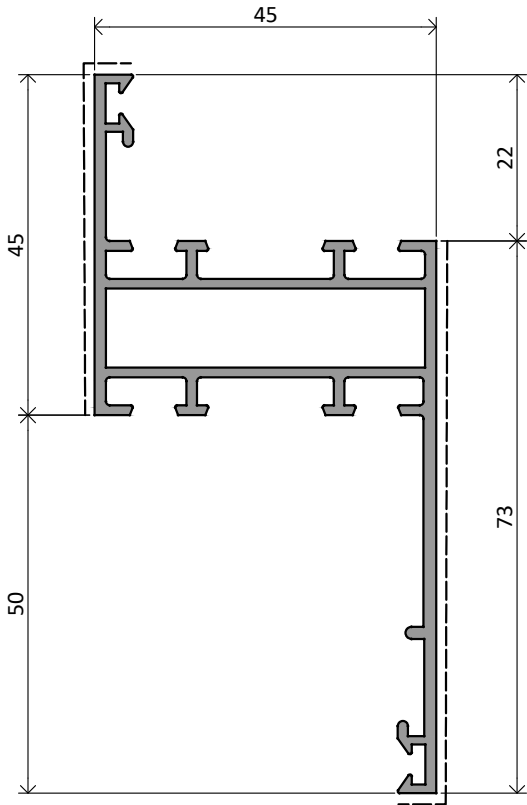
NX2770 | 1,123 Kg/m
