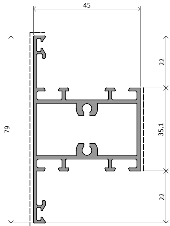
NX419 | 1,171 Kg/m
