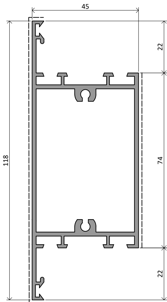
NX3704 | 1,628 Kg/m
