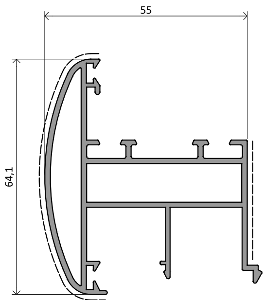
NX3767 | 1,171 Kg/m
