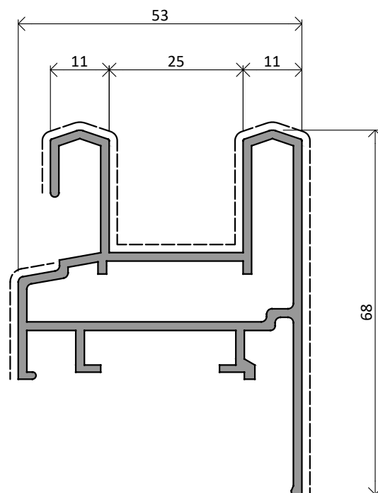
NX3790 | 1,238 Kg/m
