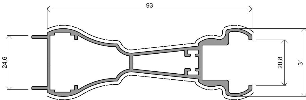
NX4019 | 1,150 Kg/m
