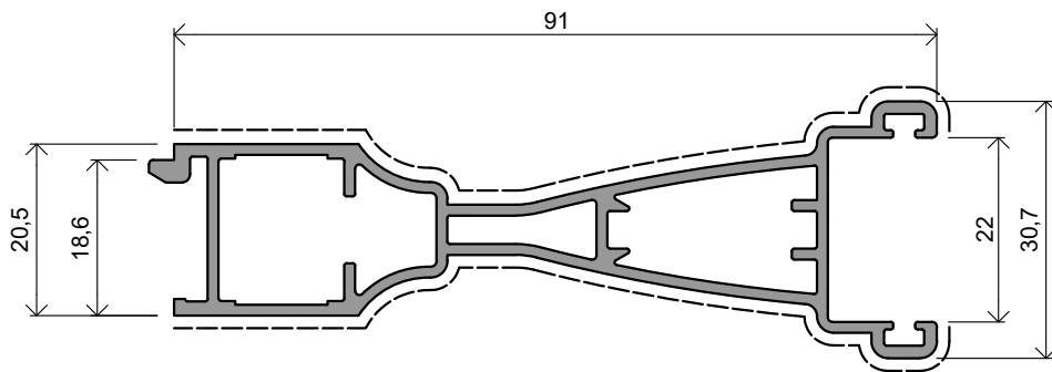
NX10014 | 1,026 Kg/m
