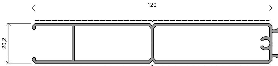
NX4018 | 1,097 Kg/m
