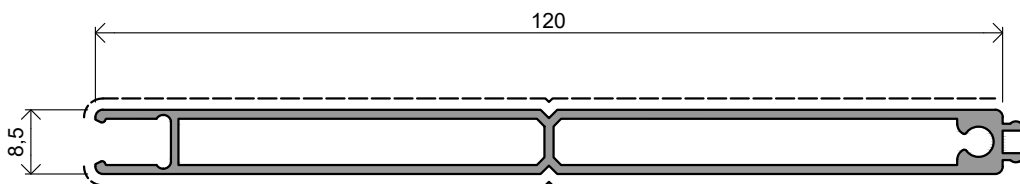
NX10015 | 1,002 Kg/m
