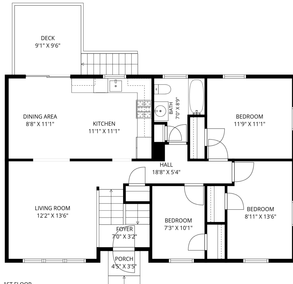
1ST FLOOR
