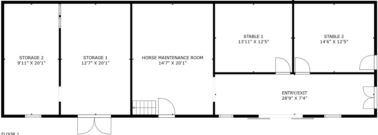
FLOOR 1
