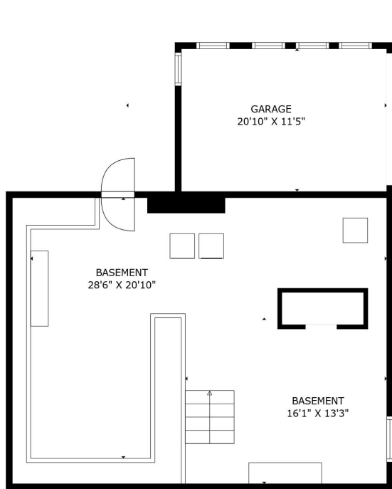
BASEMENT
