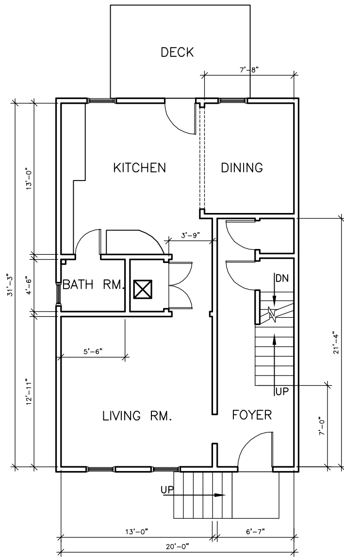
EXIST'G 1ST FLOOR PLAN 625 S.F.
