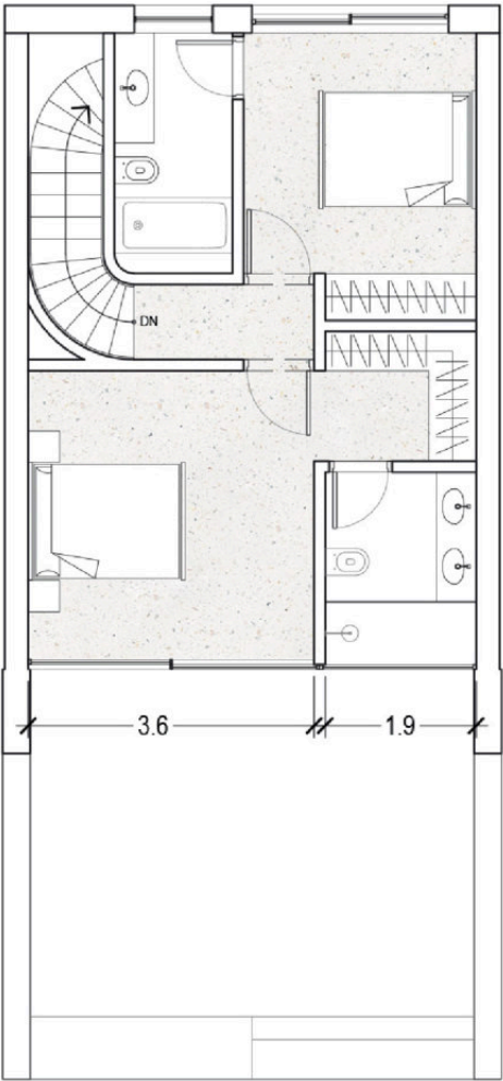
UPPER FLOOR
