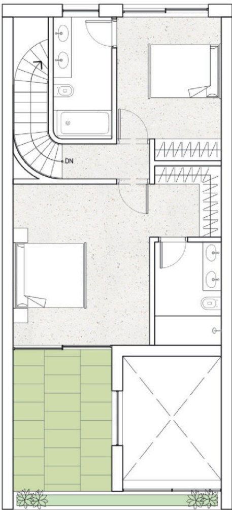
UPPER FLOOR
