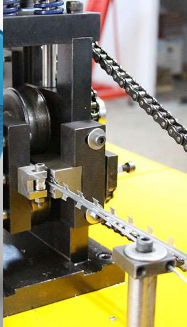
Razor Wire Production Line
