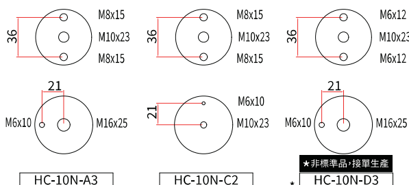
HC-10N-A3
