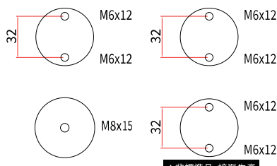
HC-50L-B1
