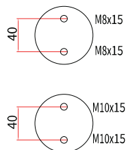
HC-70L-A1
