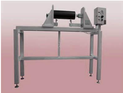
Idler axial displacement tester
